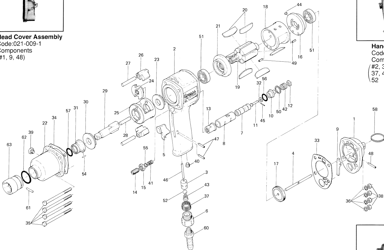
Hammer Casing Assembly Code:026-007-3 Components (#22,31,39,54,57)
