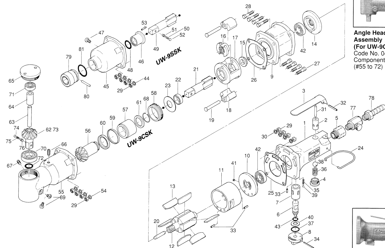
Handle Assembly Code No. 043-982-2 Components (#1, 2, 3, 4, 6, 7, 8, 31, 32, 33, 34, 35, 36, 37, 38, 39, 40, 43)
