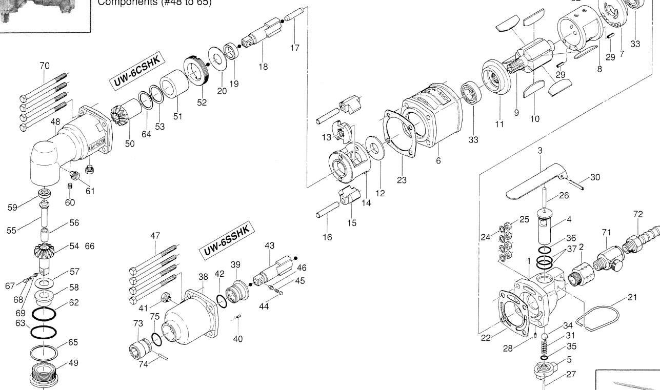
Hammer Casing Assembly (For UW-6SSHK) Code: 026-007-3 Components (#38 to 42)
