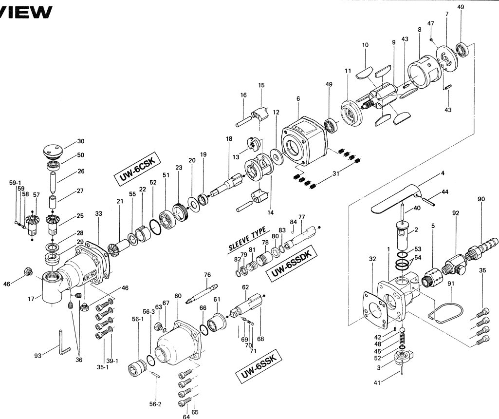
Angle Head Casing Assembly Code No. 014-883-1 Components (#17, 21, 22, 23, 24, 25, 26, 27, 28, 29, 30, 36, 46, 50, 51, 52, 55)
