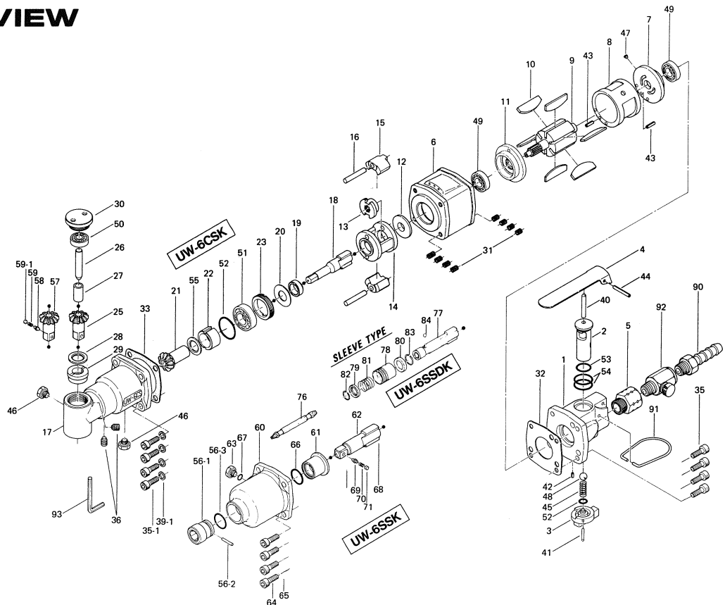
Angle Head Casing Assembly Code No. 014-883-1 Components (#17, 21, 22, 23, 24, 25, 26, 27, 28, 29, 30, 36, 46, 50, 51, 52, 55)
