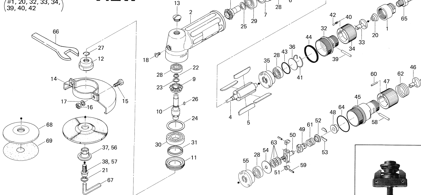
Governor Cage Assembly for USG-4S Code No. 510-893-7 Components (#49, 50, 51, 52, 53, 59, 61, 63)
